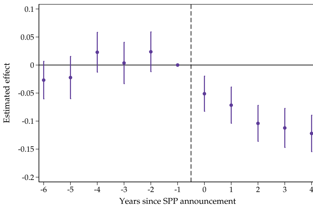
Figure A12. Event Study Estimates Exploiting Distance to Nearest SPP-Eligible Institution
